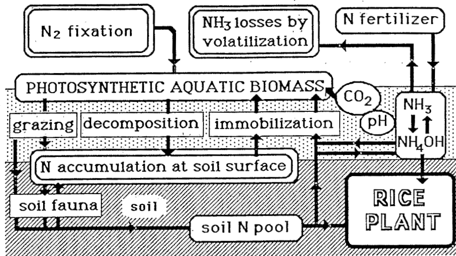
Fig. 1: Nitrogen dynamics in relation to the activity of the photosynthetic aquatic biomass in a rice field (after Roger 1986).
